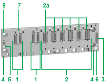
BMEXBP0602 backplane
