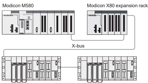
Premium X-bus expansion example
