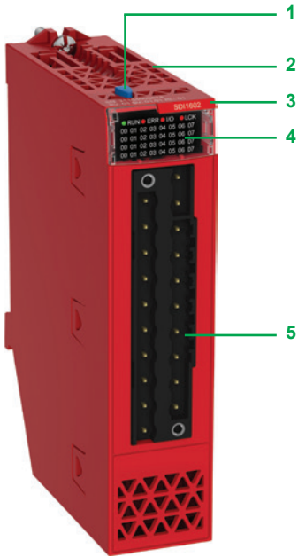
Safety discrete I/O module
